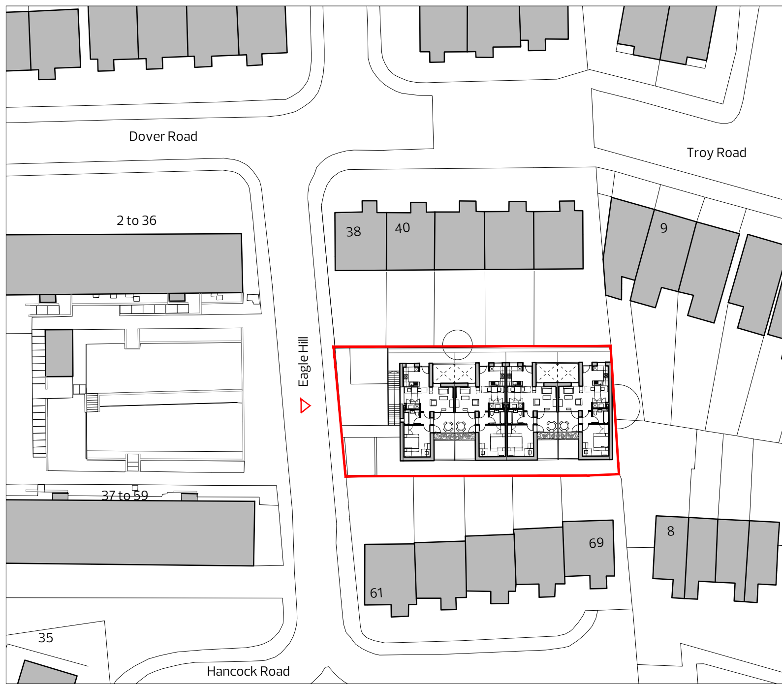
01_PROPOSED SITE PLAN
