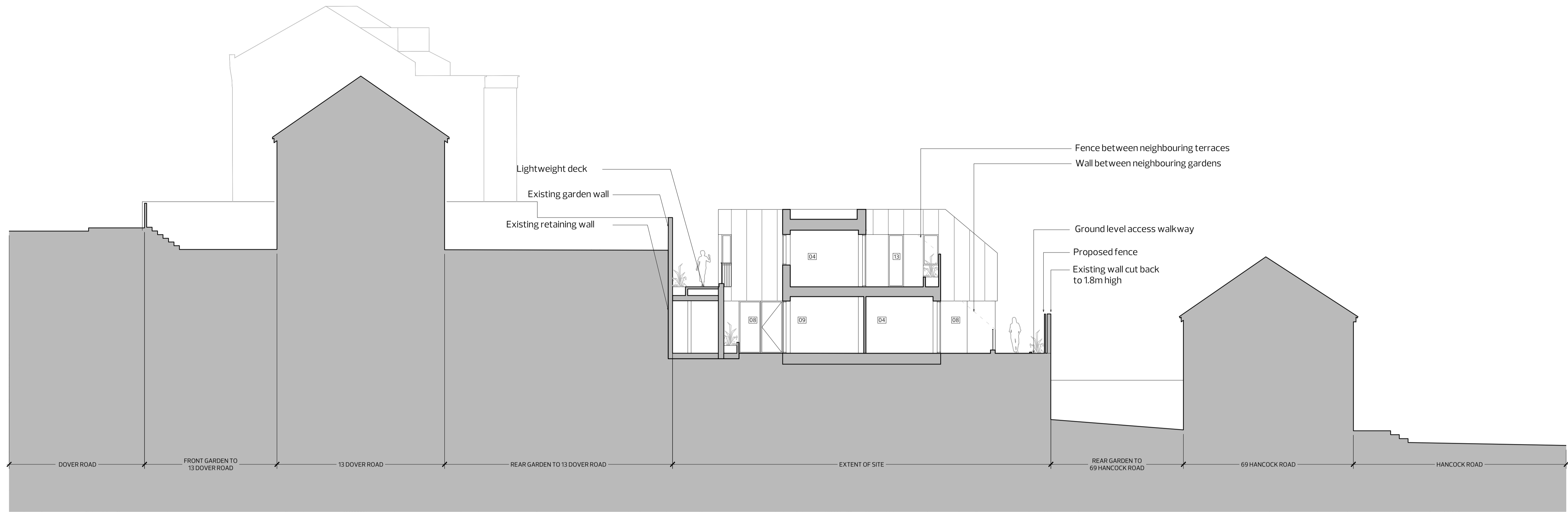
01_ PROPOSED SECTION AA
